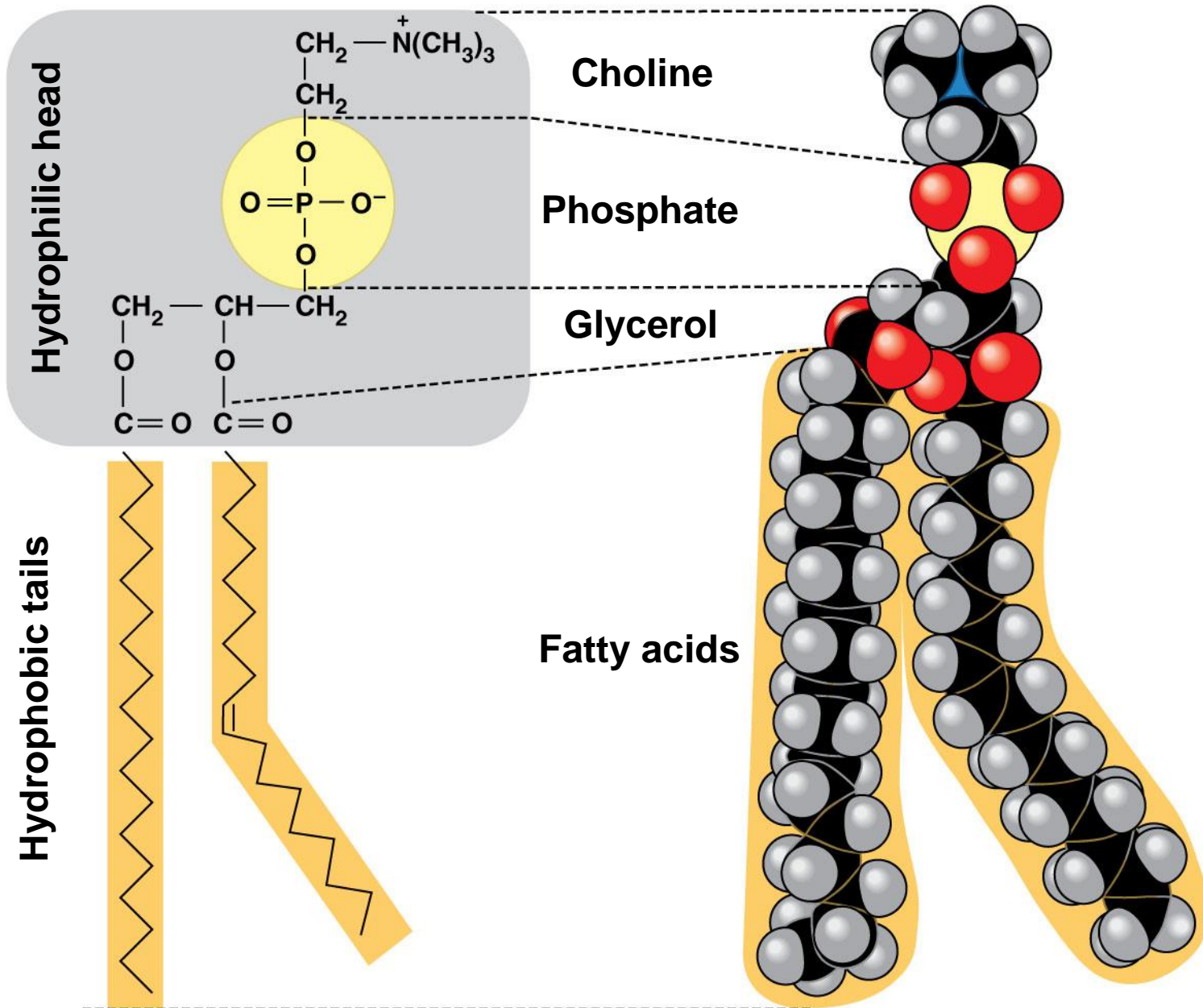
(a) Structural formula
