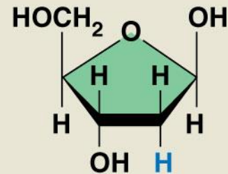
Deoxyribose (in DNA)
